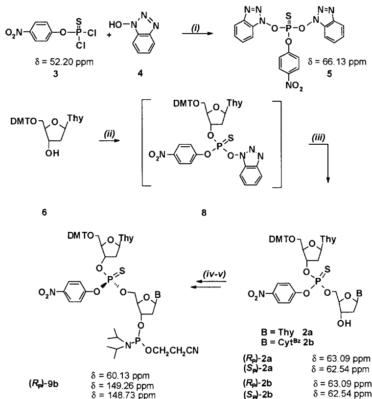
Scheme 1. Reagents and conditions: (i) 4 (2.1 equiv.), pyridine, room temp, 0.5 h; (ii) 6 in pyridine/dioxane, added dropwise, room temp, 1 h; (iii) nucleoside ( N -protected) 7 (1.1 equiv.), Me-Imi (4 equiv.), room temp, 1.5 h; (iv) silica-gel column chromatography and separation of diastereomers; (v) phosphitylation: ( i Pr 2 N) 2 POCH 2 CH 2 CN (2 equiv.), 1 H -tetrazole (4 equiv.), MeCN, 1 h; silica-gel column chromatography purification.
