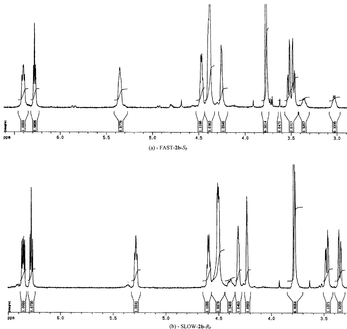
Figure 1. ^1\text{H} NMR spectra (500 MHz, in \text{CDCl}_3 ) of (a) FAST-2b and (b) SLOW-2b.
