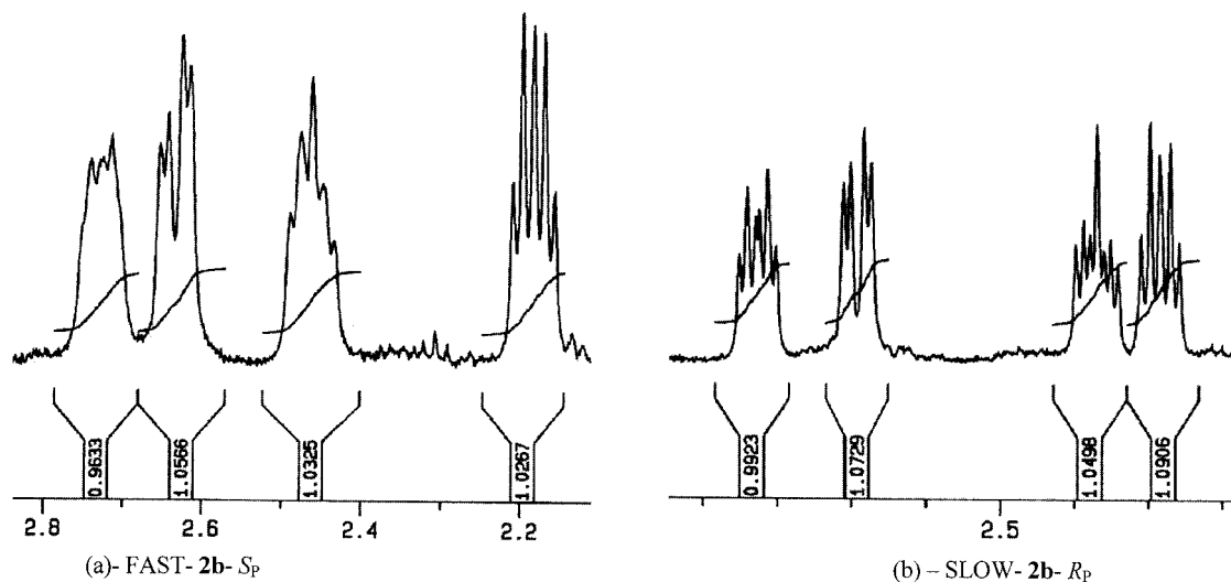
Figure 2. Fragment of ^1\text{H} NMR spectra (500 MHz, in \text{CDCl}_3 ) showing the \text{H}_{2'} region of (a) FAST-2b and (b) SLOW-2b.
