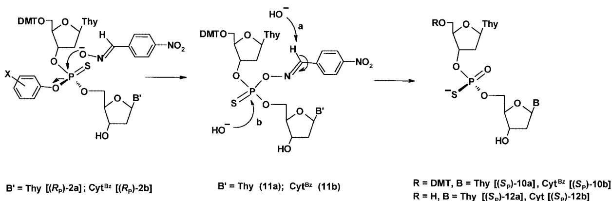
Scheme 2. Oximate-mediated removal of aryl protecting groups; path a: base-catalyzed \beta -elimination of 4-nitrobenzonitrile from the oxime ester 11 (retention of configuration); path b: hydrolysis of the oxime ester 11 (inversion of configuration).
